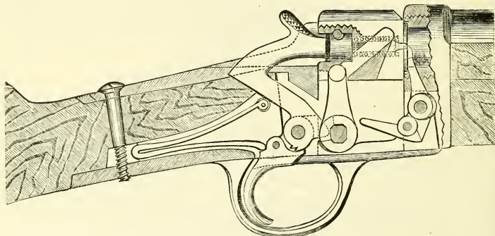
Section of the Field Rifle.—Sliding-block Pattern.
